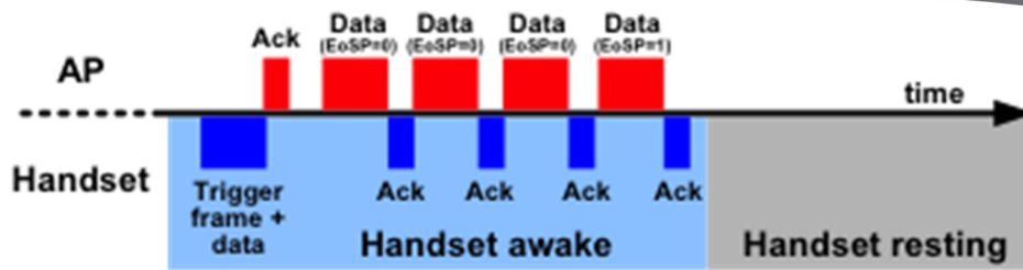
Figure 8 - WMM Power Save Timing
